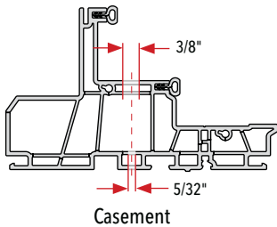
Casement
