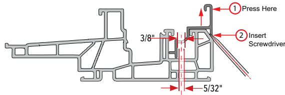
Remove sill riser (if applicable) Double/Single Hung
