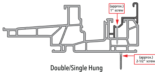
Remove sill riser (if applicable) Double/Single Hung
