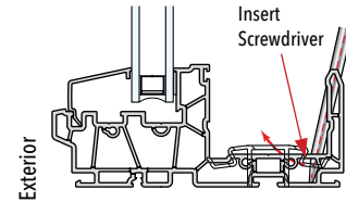
Remove vent track (if applicable) Sliding Window
