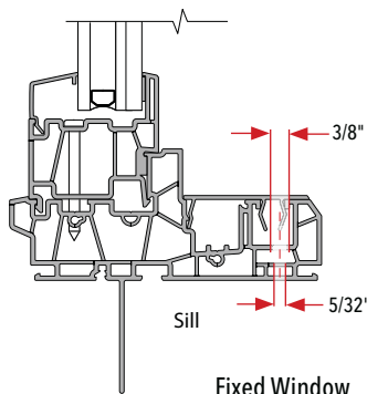
Fixed Window
